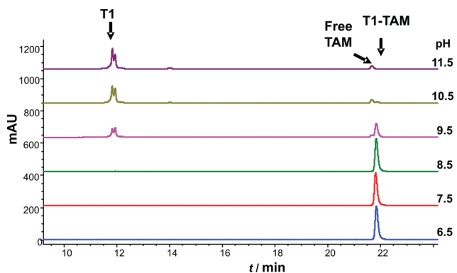
Fig. 2 Hydrolytic stability of the fluorescent TAMRA thioester, T1-TAM : HPLC chromatograms of T1-TAM after 48 h incubation at 38 °C in universal buffer at indicated pH.
