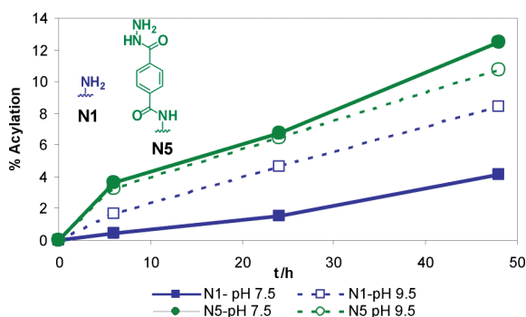
Fig. 6 Comparison between reactivities of amine- and hydrazide-modified oligonucleotides as functions of pH. Time courses of acylation reactions, monitored by HPLC, using N1 and N5 nucleophiles in 100 mM sodium phosphate buffer at the indicated pH.
