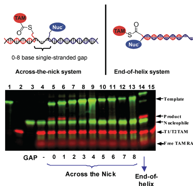
Fig. 5 DNA architectures and acyl transfer efficiency. Lane 1: S5 (template oligonucleotide); lane 2: T1-TAM ; lane 3: N1 ; lane 4: T1-TAM + N1 control (no template); lanes 5–13: T1-TAM + N1 in the presence of a template oligonucleotide incorporating a 0–8 nucleotide single-stranded gap (oligonucleotides 5–13, ESI†); lane 14: T2-TAM + N1 (end-of-helix architecture); lane 15: T2-TAM . Reactions were carried out in 100 mM sodium phosphate buffer, 100 mM NaCl, pH 9.0, 10% THF at 38 °C for 24 h.
