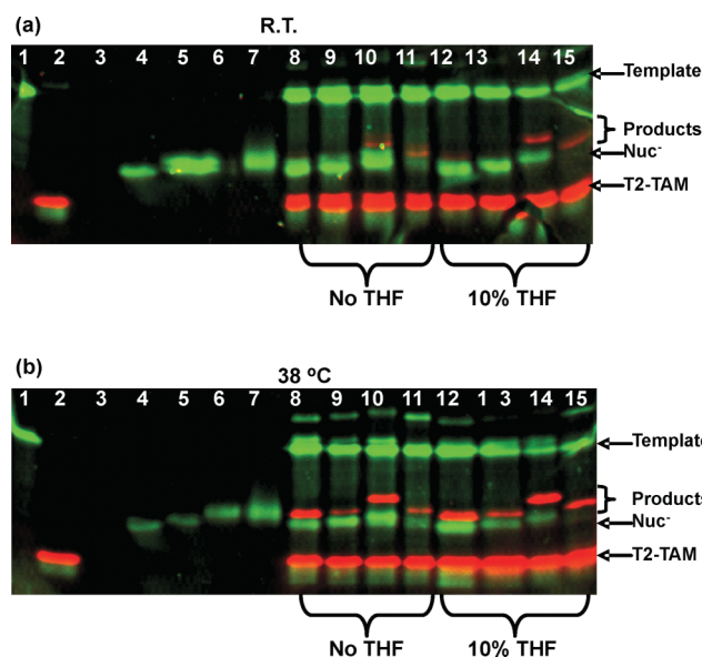
Fig. 4 Comparison between acyl transfer reactions at room temperature (R.T.) and at 38 °C. Acyl transfer reactions were carried out for 24 h in 100 mM sodium phosphate buffer, pH 8.5, with (lanes 12–15) and without (lanes 8–11) 10% THF at R.T. (a) and at 38 °C (b). Lane 1: Template oligonucleotide S5 ; Lane 2: T1-TAM ; Lane 3: blank; Lane 4: N1 ; Lane 5: N2 ; Lane 6: blank (a)/ N5 (b); Lane 7: N9 ; lanes 8–15: acyl transfer reactions with the nucleophiles as in lanes 4–7. Red channel: TAMRA (Ex532/Em605 nm); green channel: SybrGold DNA stain (Ex488/Em530 nm).
