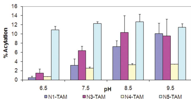
Fig. 7 Comparison of yields of acyl transfer products, using nucleophiles N1 , N3–N5 , determined from peak areas in HPLC chromatograms. Acylation reactions were carried out in 100 mM sodium phosphate buffer, 100 mM NaCl, at pH 6.5–9.5 for 48 h at 38 °C. Product peaks were identified by simultaneous measurement of TAMRA fluorescence and A_{260} .
