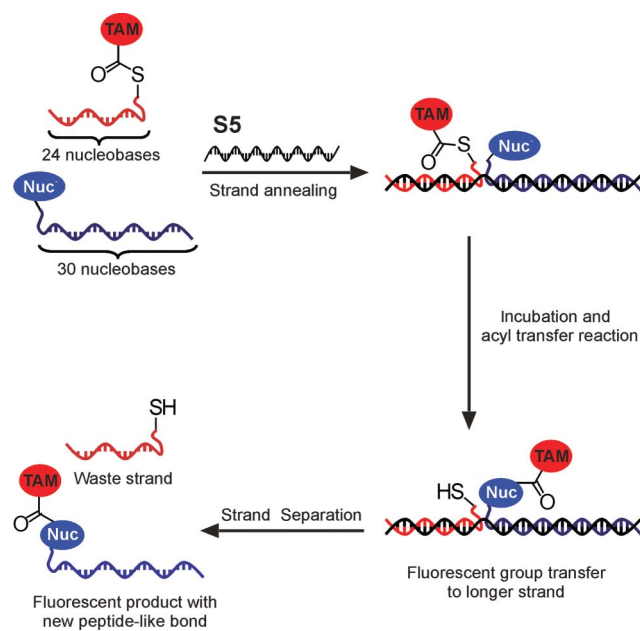
Scheme 1 DTS system for monitoring acyl transfer reactions.
